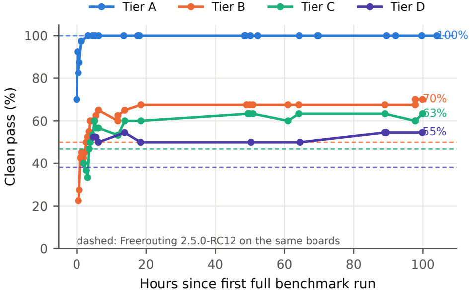
Figure 7: Clean pass of every full benchmark run (20 or more boards) since the first one, including side-by-side experiment arms. Dashed lines: Freerouting 2.5.0-RC12 on the same boards. Small run-to-run differences come from the wall-clock limit.
