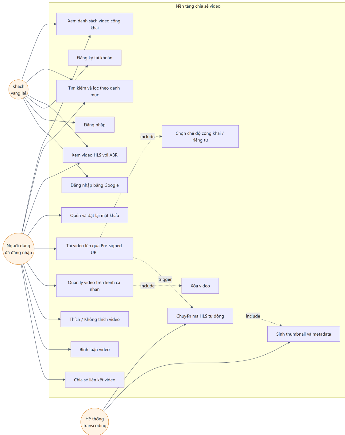
Figure 3.1: Use case diagram of the video sharing platform
