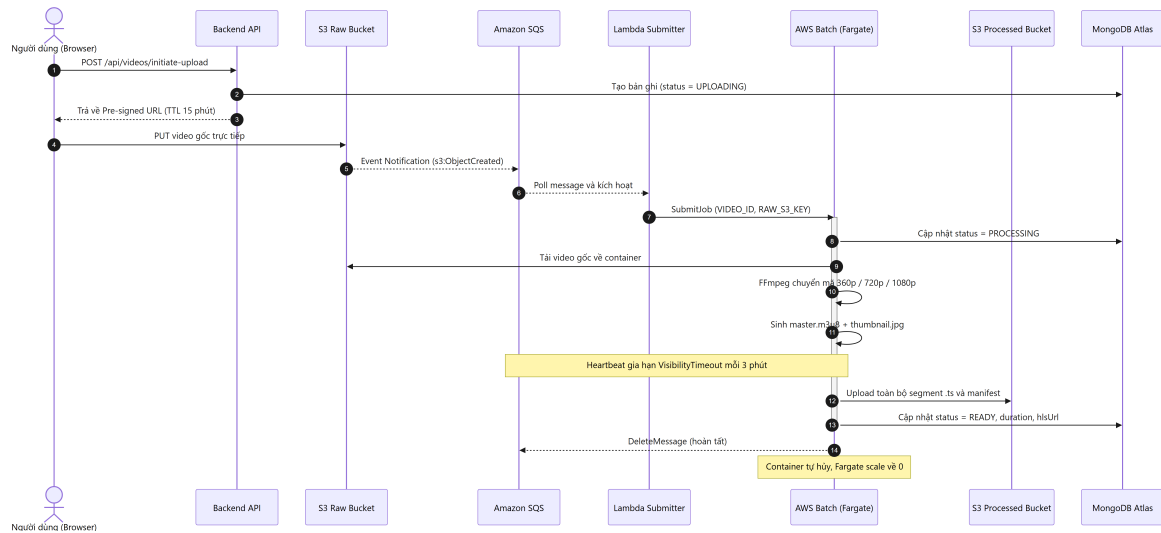
Figure 4.2: Sequence diagram of the event-driven transcoding pipeline
