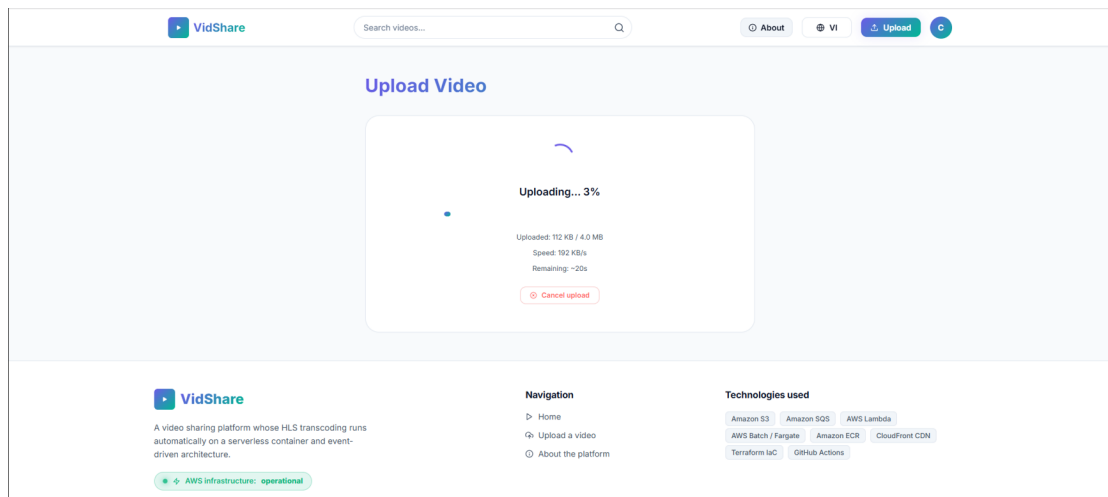
Figure 6.3: Upload page, showing direct-to-storage transfer with live telemetry
