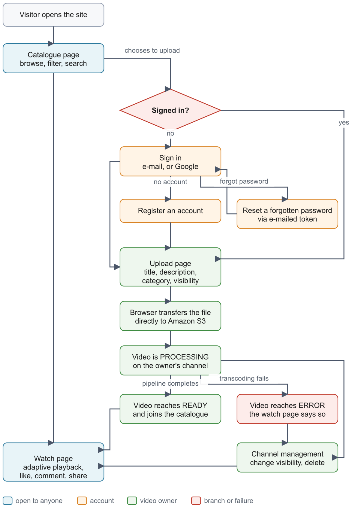
Figure 4.4: User flow through the application, from an anonymous visit to a published video
