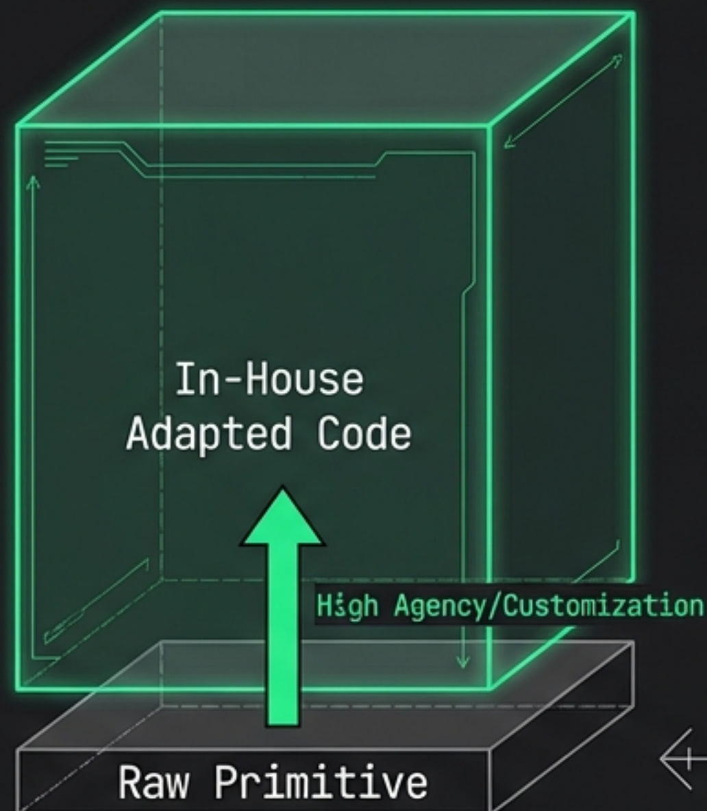
Agentic Dev
