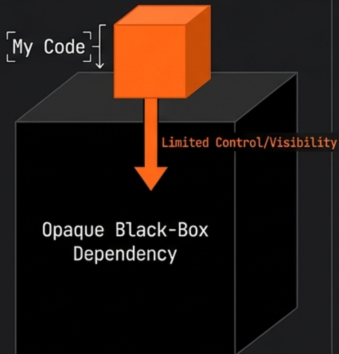
Traditional Dev
