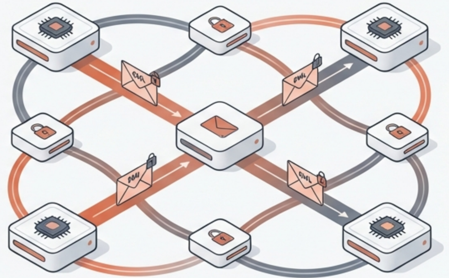
Agent pods
