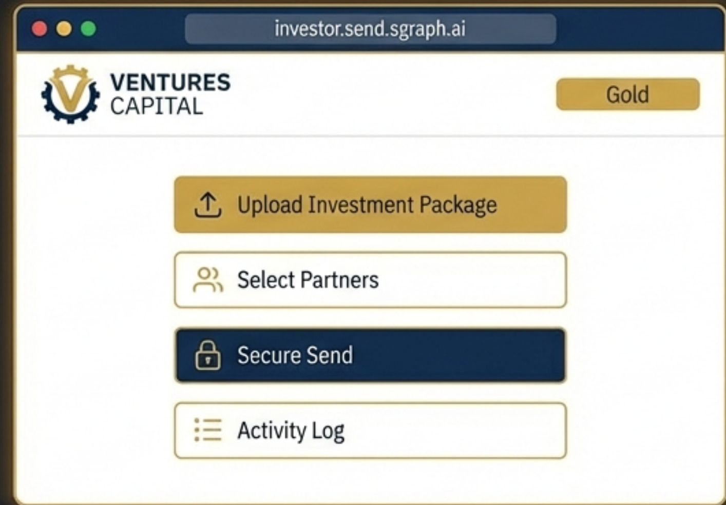
INVESTOR INSTANCE
