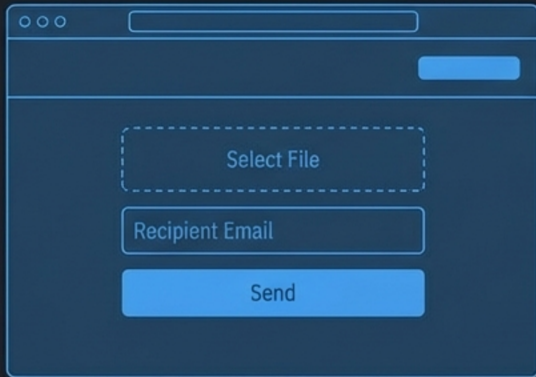
GENERIC SG/SEND
