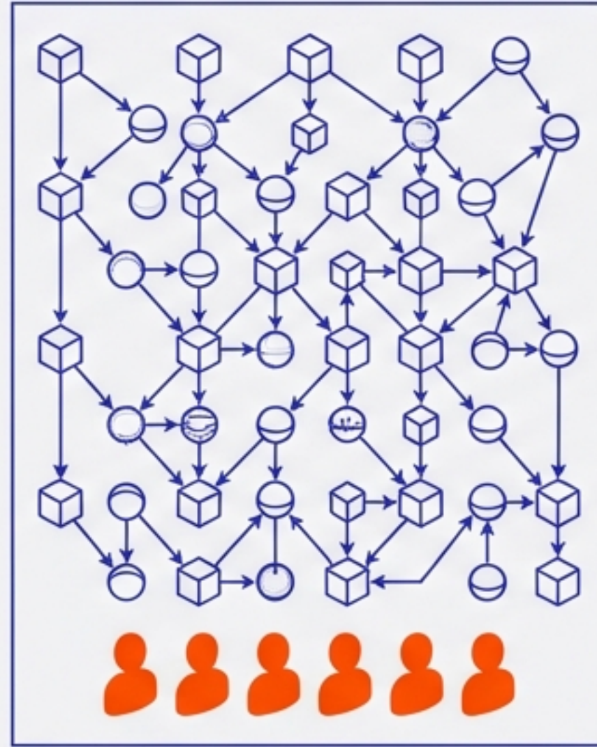
Agentic Model
