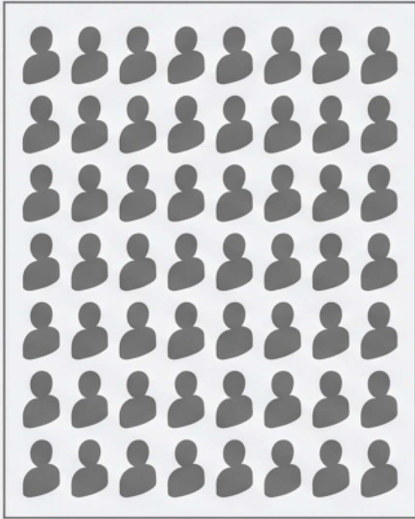
Traditional Model
