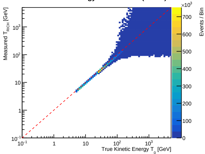
Kinetic Energy Correlation (RICH)
