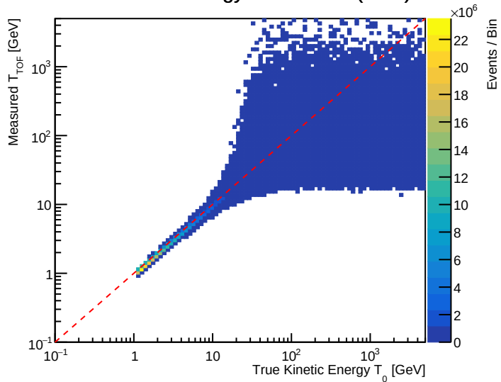
Kinetic Energy Correlation (TOF)
