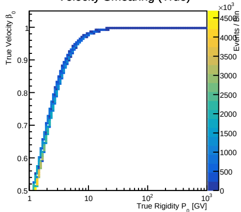
Velocity Smearing (True)
