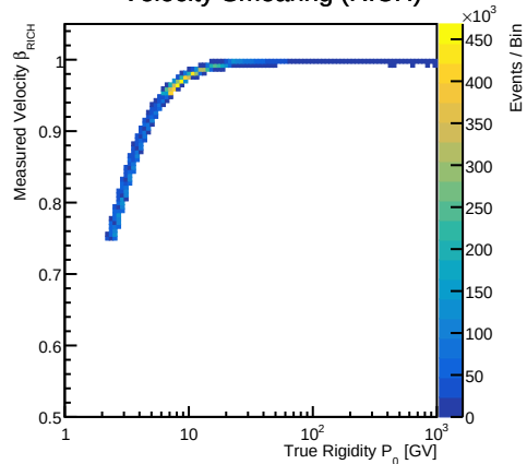
Velocity Smearing (RICH)
