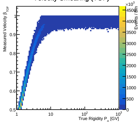
Velocity Smearing (TOF)
