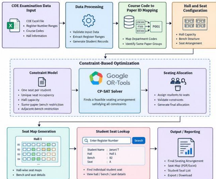
Figure 3.1 – System Architecture
