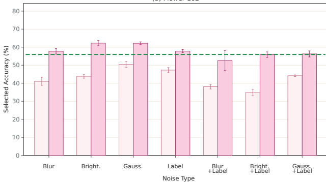
(b) Flower-102
