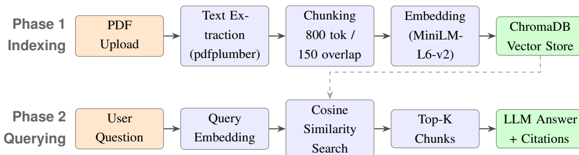
Figure 1: Two-phase RAG architecture. Phase 1 indexes each document once (top row); Phase 2 handles every user query (bottom row). The dashed arrow shows the vector store serving both phases.
