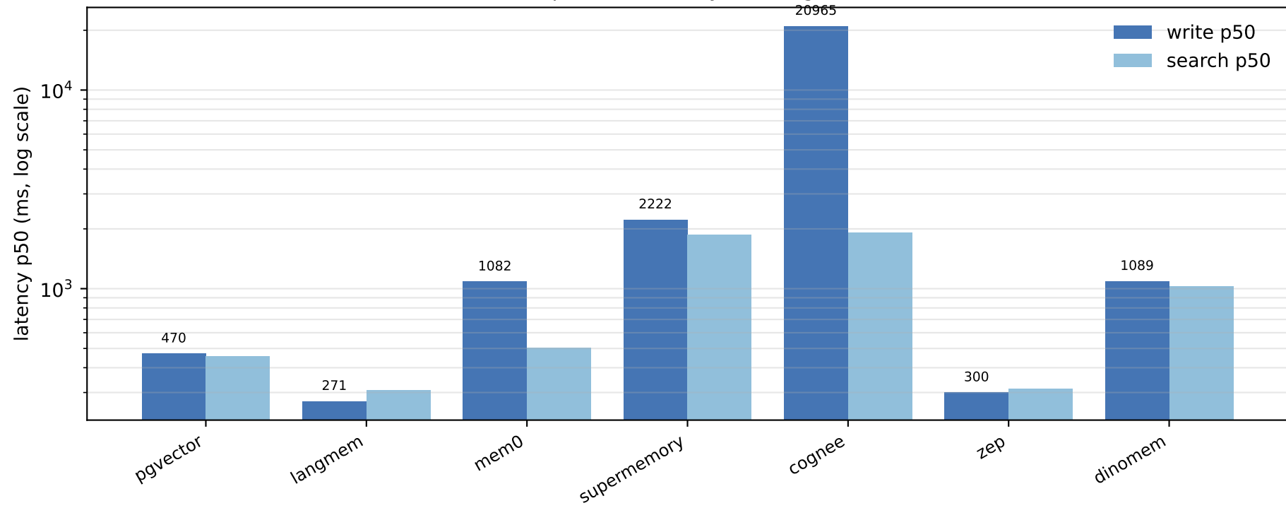
Per-operation latency (S7), log scale
