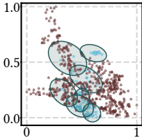
variance-kurtosis View
