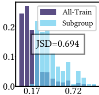
Log-loss
