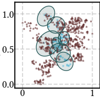
variance-skewness View
