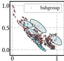
skewness-kurtosis View
