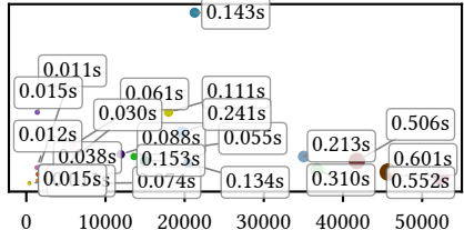
Pocket Size = 32
