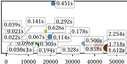
Pocket Size = 16
