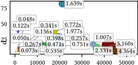
Pocket Size = 8
