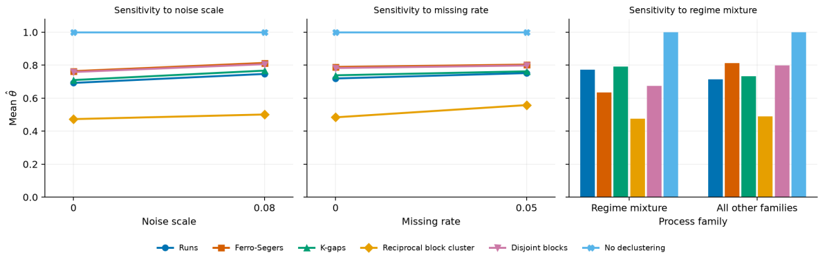
Figure 1: Estimator sensitivity to noise scale, missing rate, and regime mixture. The regime-mixture panel contrasts families rather than sweeping a parameter, since mixture is a property of the process and not a tuning knob.
