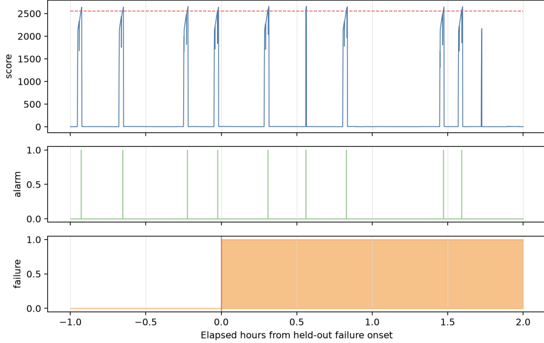
Figure 7: Traceable MetroPT held-out failure timeline. The x-axis is elapsed hours from the registered test failure onset; the panels show the fitted score threshold, alarm flags after thresholding, and labelled failure interval.
