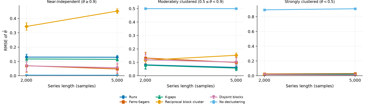
Figure 1: Finite-sample RMSE of the extremal-index estimate by series length, faceted by clustering regime. Error bars are 1.96 bootstrap standard errors. Panels use independent vertical scales because the no-declustering control has RMSE |1 - \theta| by construction. Reference values are \theta = 1 (theoretical) for the near-independent panel, \theta = 1/2 (theoretical) for the moderately clustered panel, and numerically established values below 0.3 for the strongly clustered panel.
