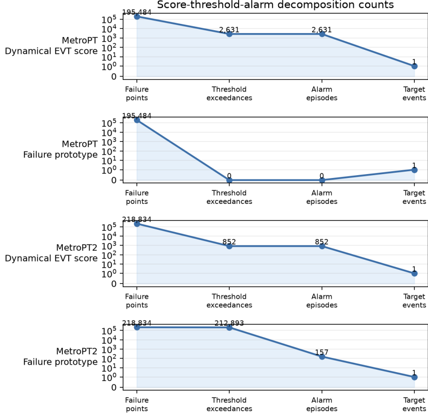
Figure 7: Score-threshold-alarm decomposition for real held-out event methods. The panels show count-valued transitions rather than mixing event precision with false alarms per day on one axis.
