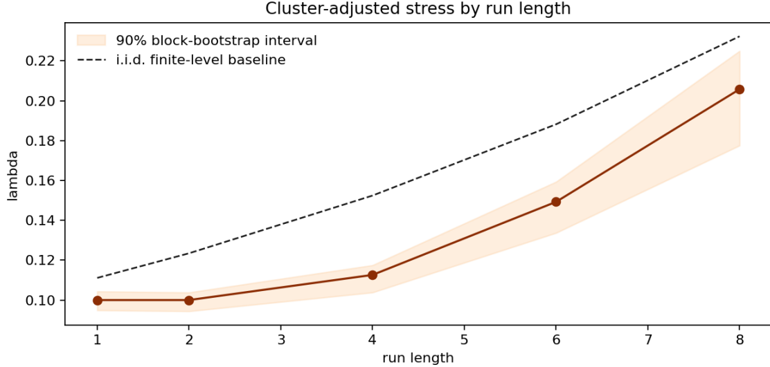
Figure 5: Run-length sensitivity of the cluster-adjusted stress functional at the 0.90 threshold quantile. The dashed curve is the finite-level i.i.d. benchmark, so the figure makes clear that raw monotonicity in r carries no persistence information by itself; only departures from the benchmark do.
