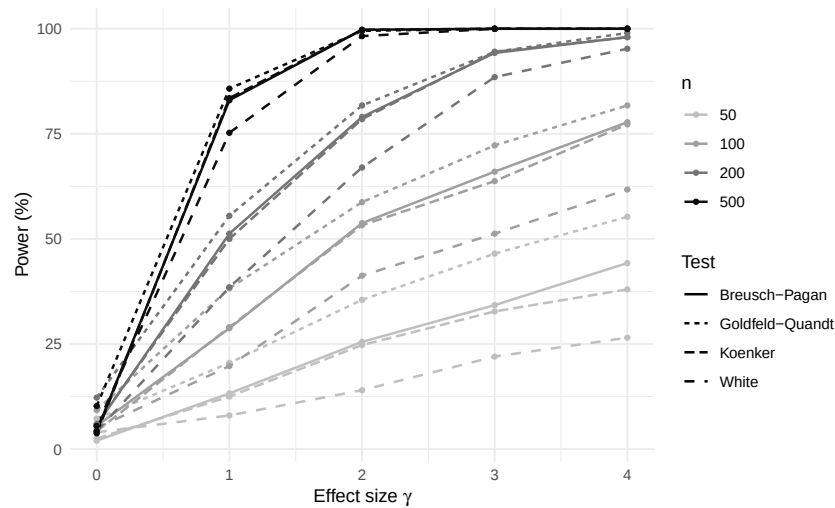
Figure 1: Power curves for detecting linear heteroscedasticity ( \sigma_i^2 = \sigma^2(1 + \gamma x_i) , x_i \sim U(0,1) , 400 Monte-Carlo replications). Line type distinguishes the tests (White, Breusch-Pagan, Koenker, Goldfeld-Quandt); sample size increases from light to dark shading ( n = 50, 100, 200, 500 ).
