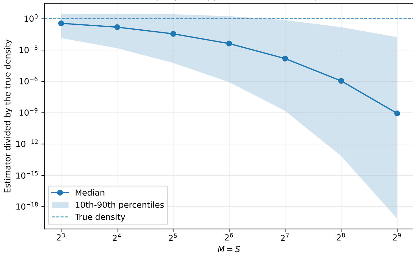
Counterexample path: typical estimates collapse to zero
