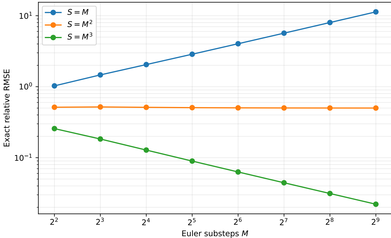
Four-dimensional Brownian motion: joint-rate comparison
