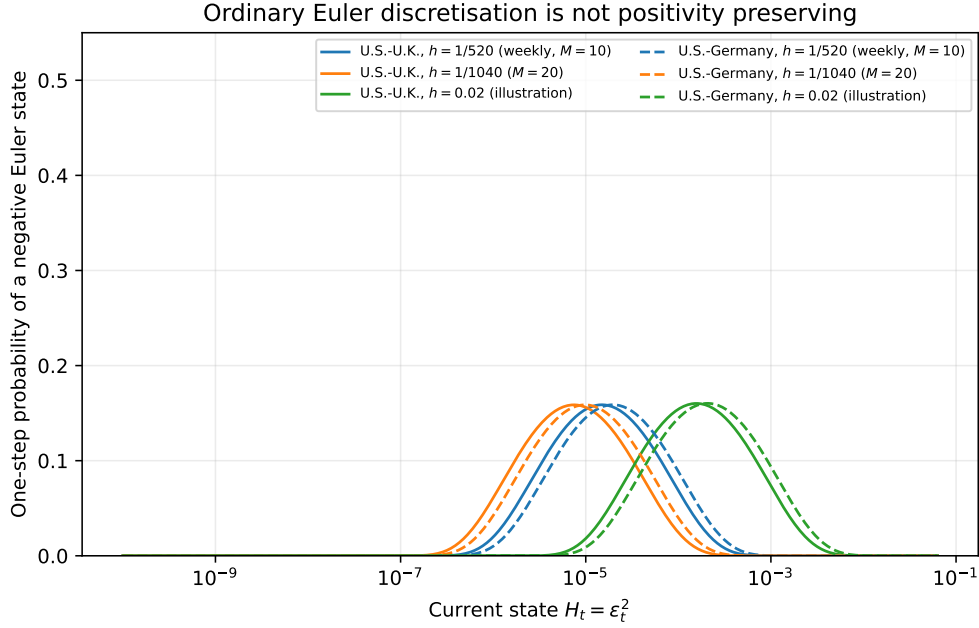
Figure 5: One-step probability that ordinary Euler discretisation of the incompleteness specification H_t = \epsilon_t^2 in (60) produces a negative state, at the estimates in Table 3 of Brandt and Santa-Clara (2002). Solid lines are the U.S.–U.K. estimates and dashed lines the U.S.–Germany estimates. The application step sizes h = 1/520 and h = 1/1040 are shown together with a coarser illustrative value. Halving h shifts each curve left and lowers its peak slightly, the maximum decreasing monotonically to \Phi(-1) \approx 0.1587 from above rather than to zero; see Proposition C.1. Three points about scope. The figure concerns direct Euler discretisation of H ; it is not a simulation of the implemented transformed chain, which substitutes \epsilon_t out and simulates (r, r^*, e, v) ; and it illustrates the boundary mechanism only. Each curve is a one-step probability conditional on the current state, so no point on it is a frequency with which any chain visits that state. See Section C.
