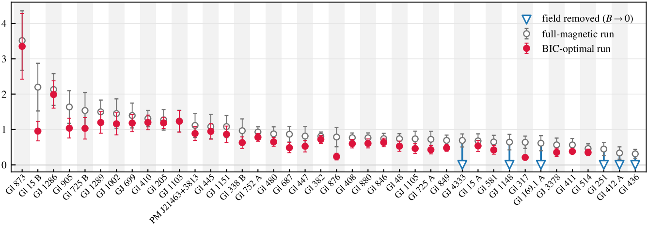
Average magnetic field \langle B \rangle (kG)
