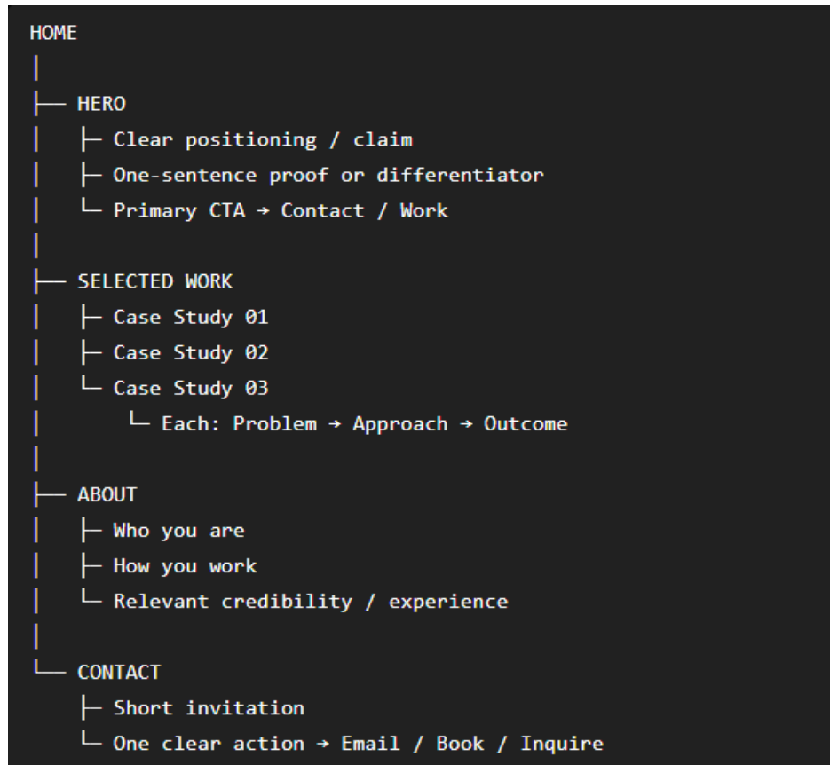
Figure 1: Portfolio Sitemap
