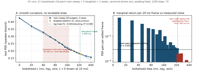
Fig. 1. Dense sweep, canonical-phone arm, 2 seeds: the 16-point main sweep (circles) with the five targeted saturation-region additions (diamonds). Left: smooth curvature; the shaded band spans the breakpoint estimates produced by three defensible treatments of L=0 , none identifiable. Right: marginal return per added 20 ms frame against the measured 2\sigma floor; red bars are below it.
