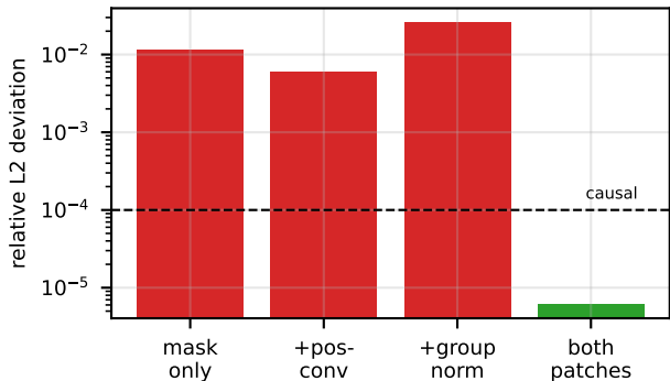
Truncation proof: only both patches are causal
