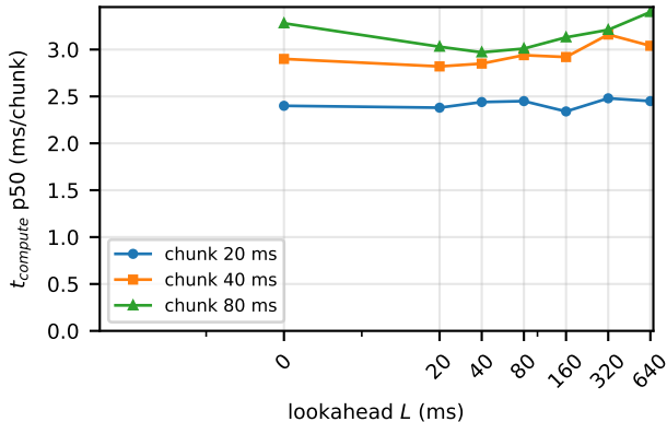
Compute is flat in lookahead (Apple M4)
