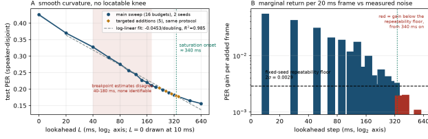
Figure 1: Dense sweep, conversion arm, 16 lookaheads × 2 seeds. Left: smooth curvature; the shaded band spans the breakpoint estimates produced by three defensible treatments of L=0 , none identifiable. Right: marginal return per added 20 ms frame against the measured 2\sigma floor; red bars are below it.
