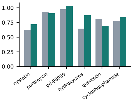
Cytoplasm:nucleus intensity
