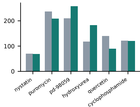
Cytoplasm:nucleus intensity
