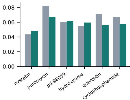
Edge/texture strength
