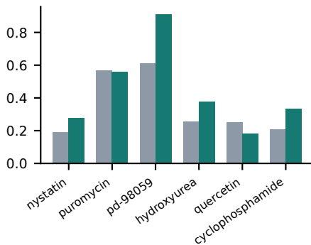
Edge/texture strength
