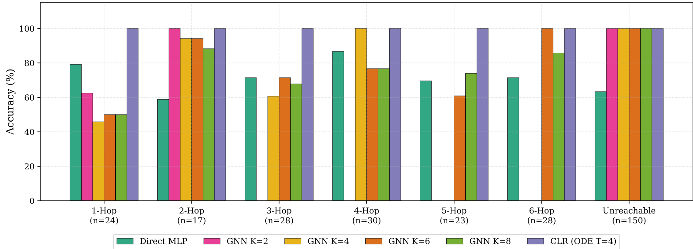
Cora Multi-Hop Reachability Breakdown by Citation Chain Length
