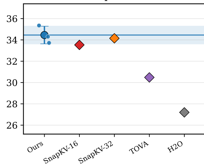
Summarization \sigma=0.40
