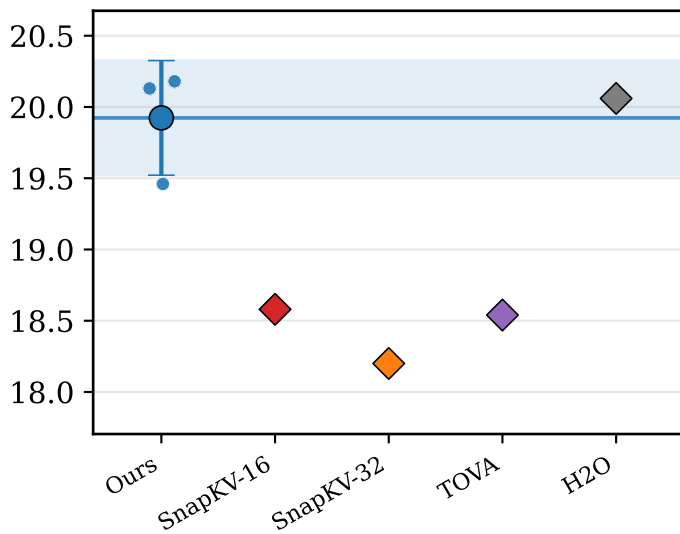
Summarization \sigma=0.40
