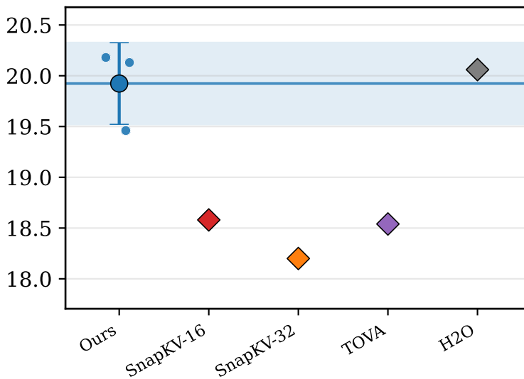
Summarization ( \sigma=0.40 )
