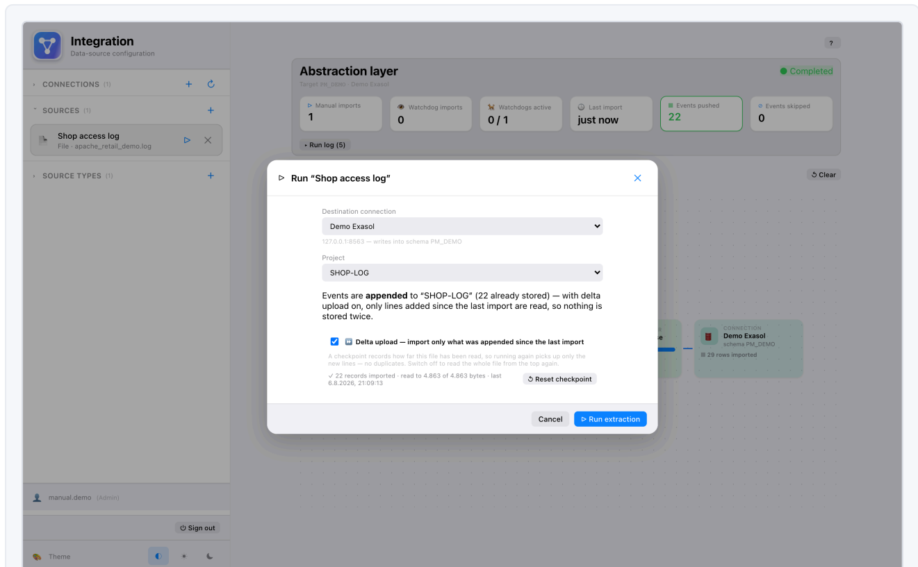
Figure 19.3 — The Run dialog. You choose the Destination connection and the Project (an existing one or a new id), leave Delta upload on to import only new lines, and press Run extraction . The checkpoint panel below records how far the file has been read.
