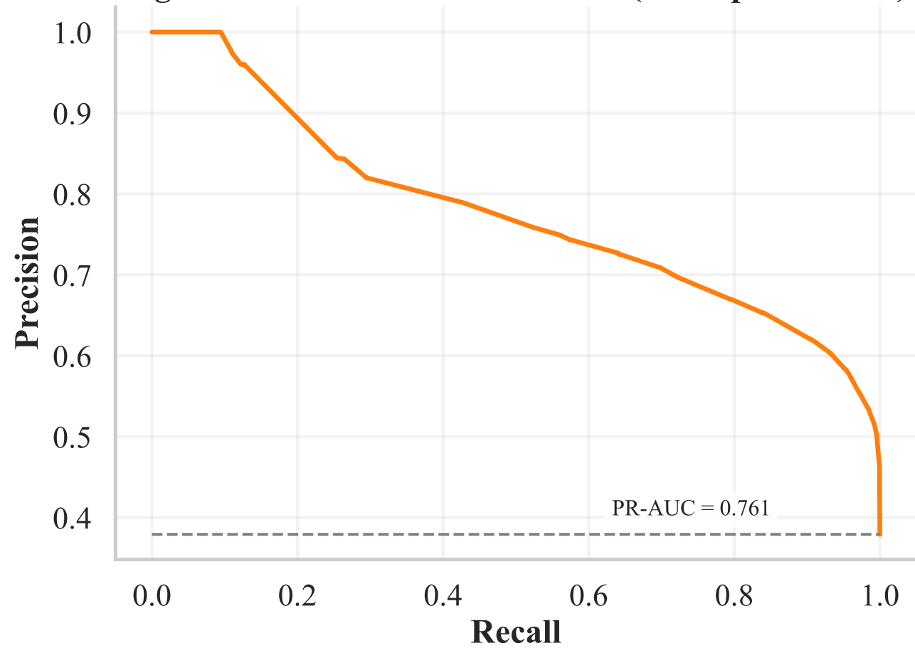
Figure 1B. Precision-Recall Curve (Champion Model)
