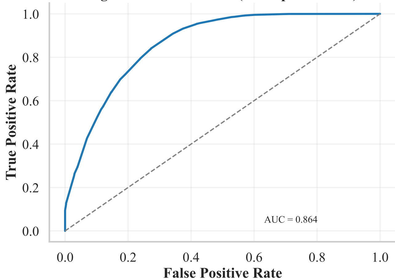
Figure 1A. ROC Curve (Champion Model)
