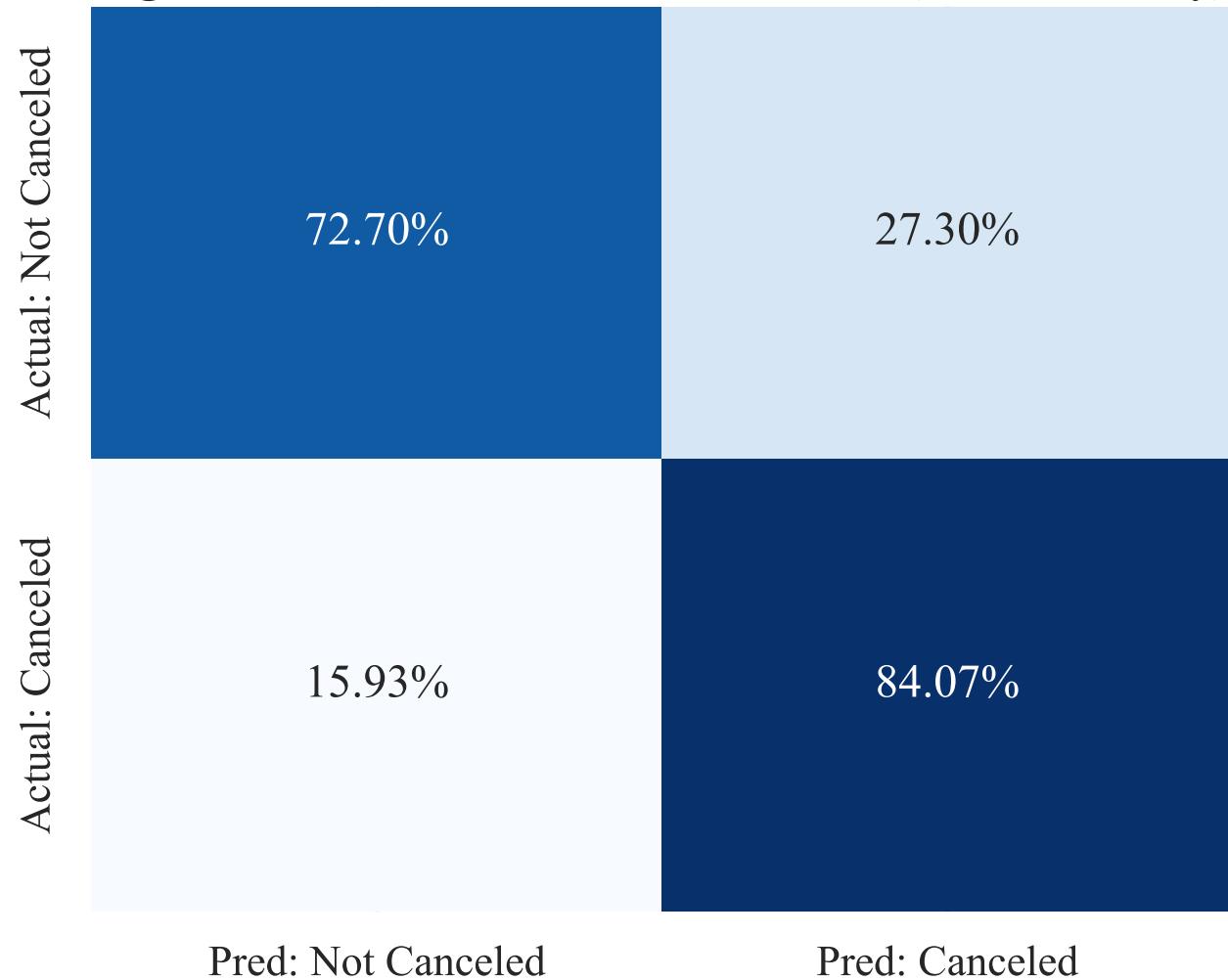
Figure 3. Normalized Confusion Matrix (Max-F1 Policy)
