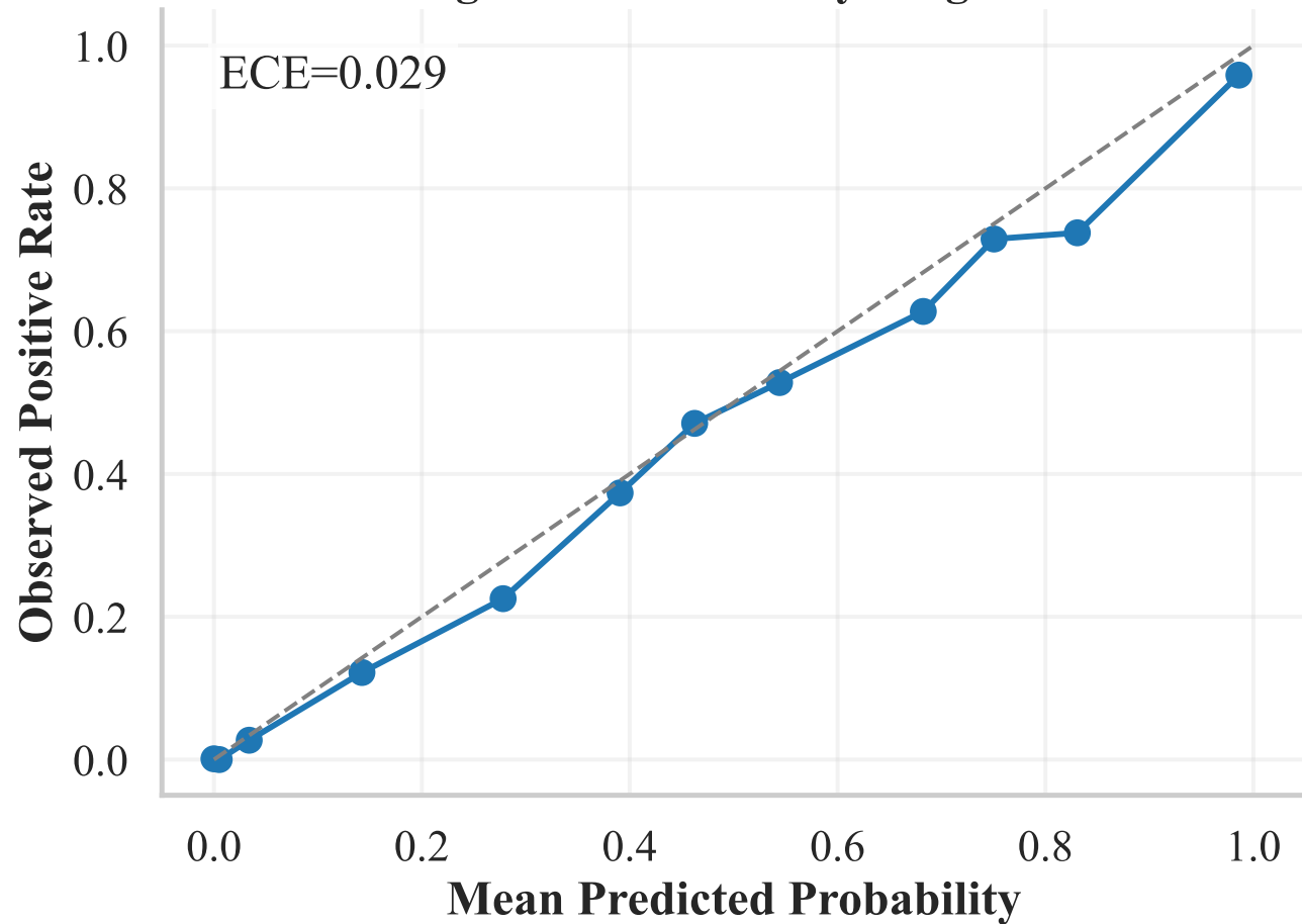
Figure 5A. Reliability Diagram
