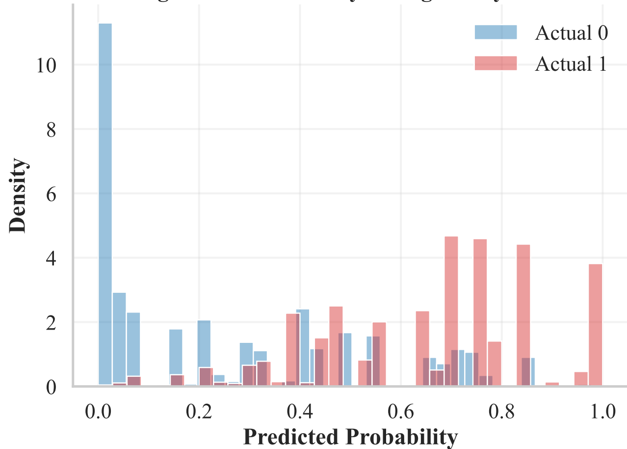
Figure 5B. Probability Histogram by Class
