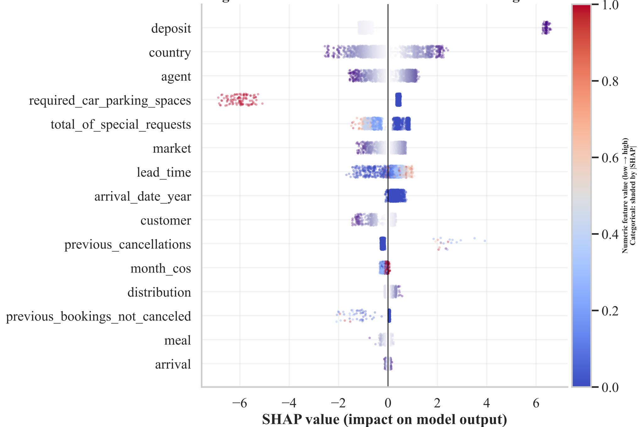
Figure 14. SHAP Beeswarm — Direction & Magnitude
