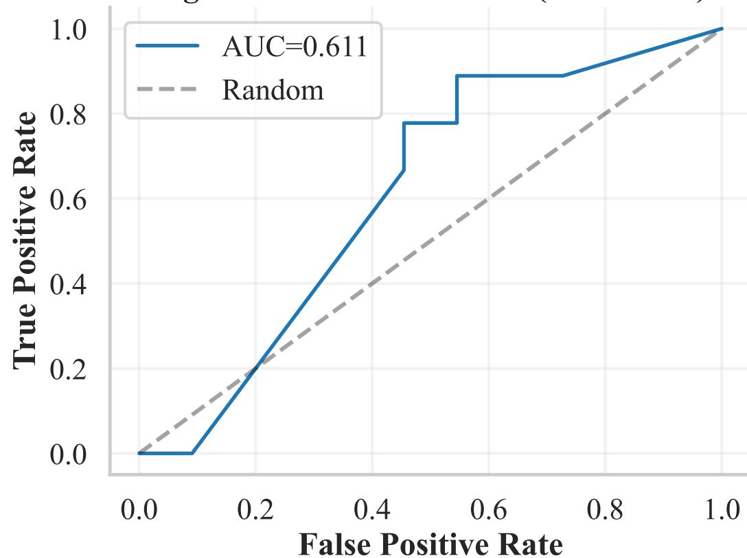
Figure 2.2A — ROC curve (PH test set)
