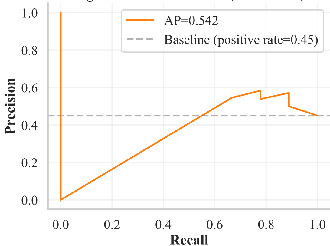
Figure 2.2B — PR curve (PH test set)
