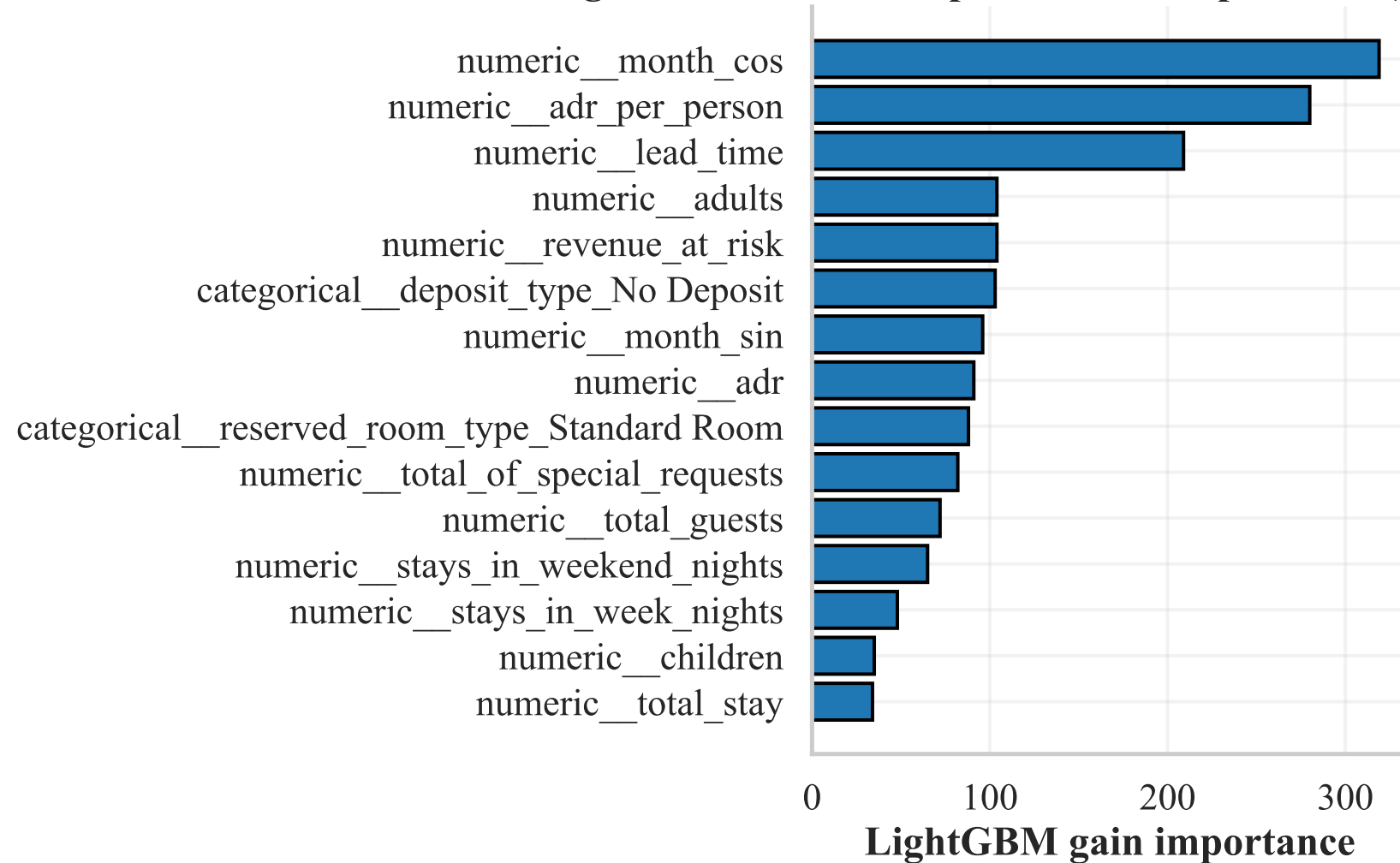
Figure 2.7 — PH champion feature importance (top 15 encoded)
