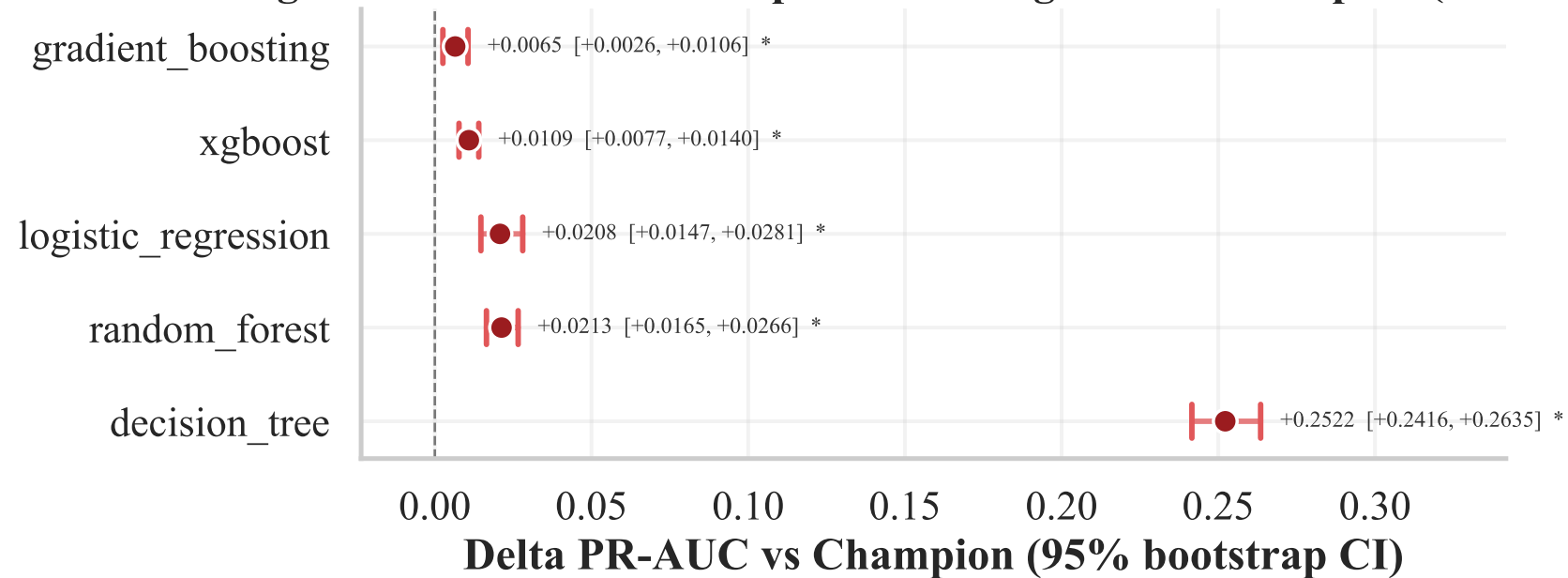
Figure 7.6 - Paired Bootstrap Deltas vs LightGBM Champion (PR-AUC)
