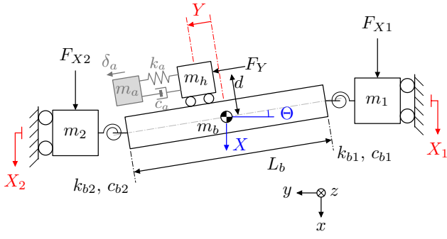
Fig. 6: Simulated gantry with a payload-mounted absorber. The light-gray elements ( m_a, k_a, c_a, \delta_a ) are absent from the baseline.
