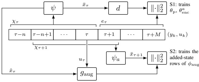
Fig. 5: Windows of PS on one record, layout adapted from [22, Fig. 2]. S1 (top): the encoder maps the window \chi_\tau to \hat{x}_\tau , and the decoder d maps its added part \bar{x}_\tau to the residuals e_\tau of the next M samples (26). S2 (bottom): g_{\text{aug}} maps \hat{x}_\tau and the recorded u_\tau to the added state encoded from the window shifted by one sample (28). [TODO: The figure shows the target from \tau + 1 , as in the final runs (FINAL-RUN-FIXES.md item 5); the current runs start it at \tau .]
