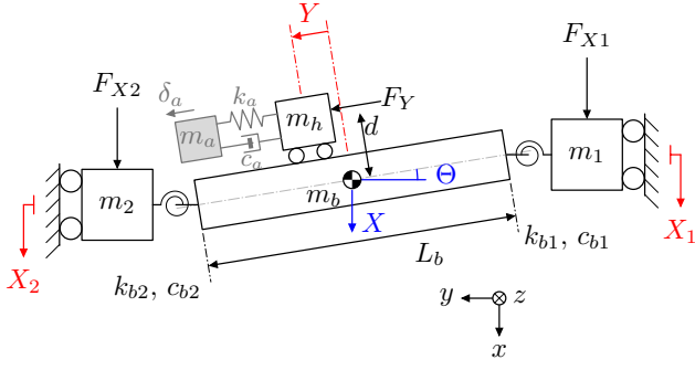
Fig. 6: Simulated gantry with a payload-mounted absorber. The light-gray elements ( m_a, k_a, c_a, \delta_a ) are absent from the baseline.
