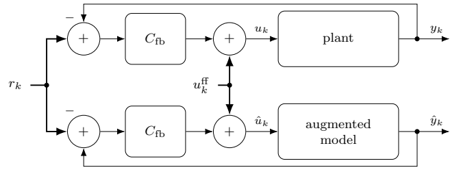
Fig. 4: Recorded plant loop (top) and augmented-model loop (bottom), driven by one shared reference r_k and feedforward u_k^{\text{ff}} , with the same feedback controller. The model output is evaluated before the input advances its state to the next sample.
