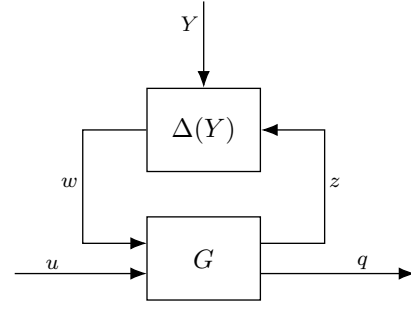
Fig. 2: [TODO: Self-scheduled baseline interconnection. The Delta-block closes the latent variables of G through w = \Delta(Y)z , with \Delta(Y) = YI_6 and Y a component of the state.]
