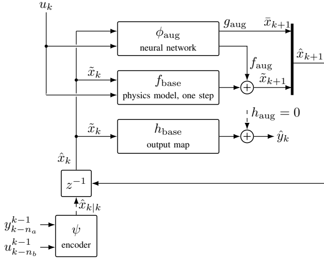
Fig. 3: Augmented model. The physics step f_{\text{base}} and the network \phi_{\text{aug}} act in parallel on \hat{x}_k . \phi_{\text{aug}} supplies f_{\text{aug}} and g_{\text{aug}} , and the output map is not learned. The encoder \psi sets \hat{x} at each window start. During training, the input is the closed-loop input of Section III-C. [TODO: No setpoint generator currently for the inputs; layout cramped at one column width.]
