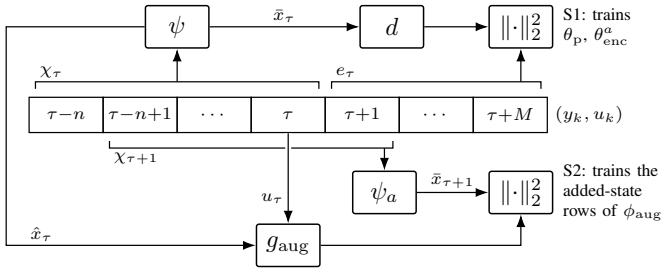
Fig. 5: Windows of PS on one record, layout adapted from [23, Fig. 2]. S1 (top): the encoder maps the window \chi_\tau to \hat{x}_\tau , and the decoder d maps its added part \bar{x}_\tau to the residuals e_\tau of the next M samples (26). S2 (bottom): g_{\text{aug}} maps \hat{x}_\tau and the recorded u_\tau to the added state encoded from the window shifted by one sample (28). [TODO: The figure shows the target from \tau + 1 , as in the final runs (FINAL-RUN-FIXES.md item 5); the current runs start it at \tau .]
