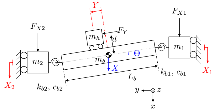
Fig. 1: [ TODO: Lumped-parameter gantry schematic adapted from the mechanical arrangement in [1]. Red labels denote actuator coordinates and blue labels generalized coordinates.]
