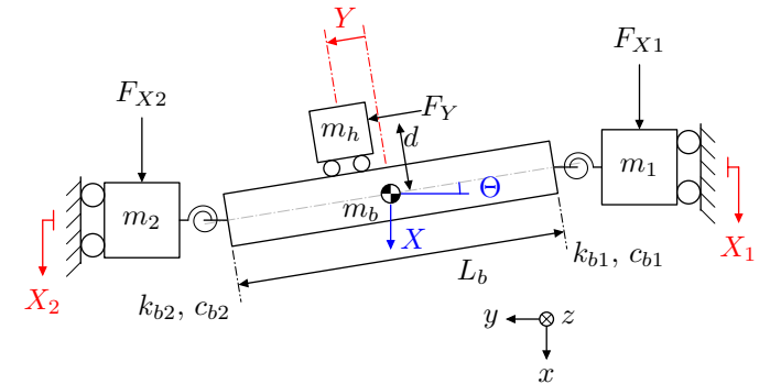
Fig. 1: Lumped-parameter gantry schematic adapted from the mechanical arrangement in [?]. Red labels denote actuator coordinates and blue labels generalized coordinates.
