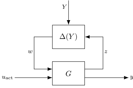
Fig. 1: Baseline as a linear fractional representation: the constant part G of (??) closed by the scheduling block \Delta(Y) = YI_6 , with z, w \in \mathbb{R}^6 and u_{\text{act}}, y \in \mathbb{R}^3 . The payload position Y is a state of G , so the model is self-scheduled.
