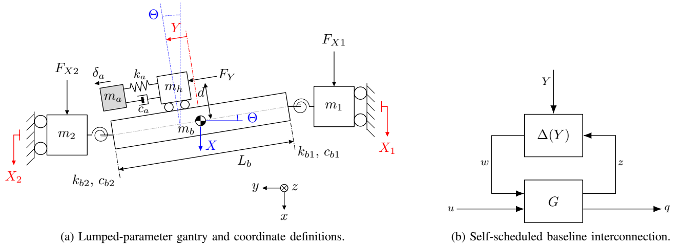
Fig. 1: Physics baseline. (a) Lumped-parameter schematic adapted from the mechanical arrangement in [1]; the absorber subsystem is present only in the simulated data-generating plant. (b) The constant interconnection G is closed by \Delta(Y) = YI_6 , where Y is a component of the state.
