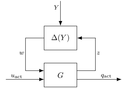
(b) Self-scheduled baseline interconnection.
