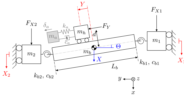
(a) Lumped-parameter gantry and coordinate definitions.
