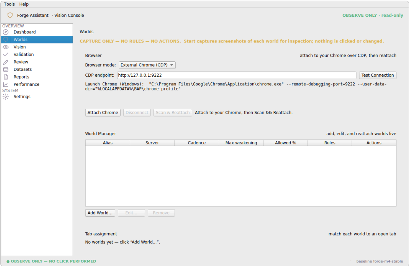
The Worlds page after choosing "External Chrome (CDP)" and restarting — Test Connection, Attach Chrome, then Scan && Reattach.
