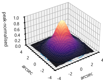
CDK 508 mm f/7.8 — M13, B
